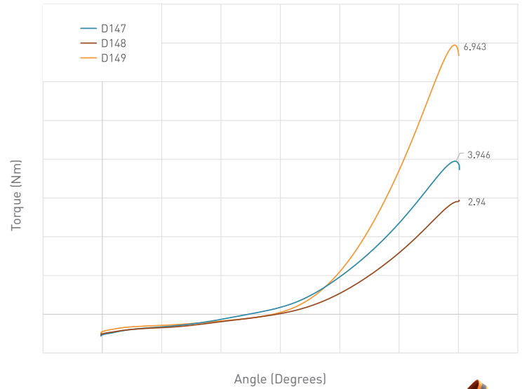
DFX 30° FORM: TORQUE/ANGLE
